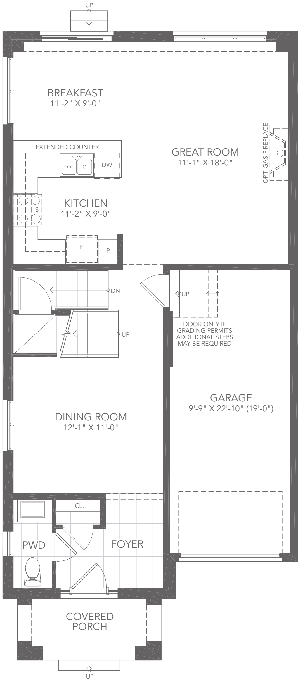
GROUND FLOOR PLAN A
