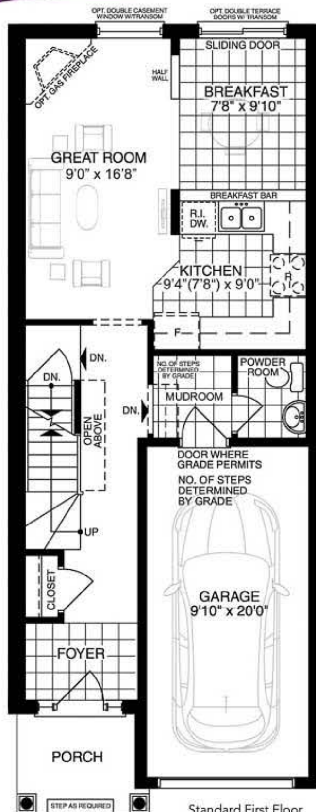
Standard First Floor
