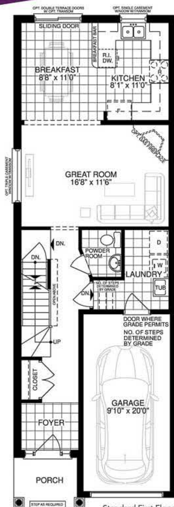
Standard First Floor
