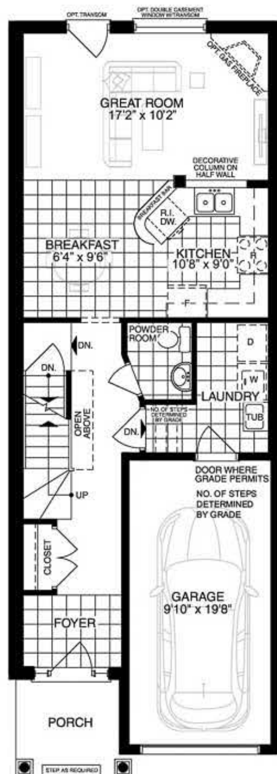
Standard First Floor
