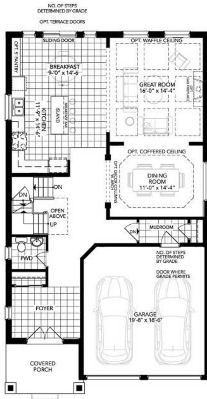
First Floor Elevation A
