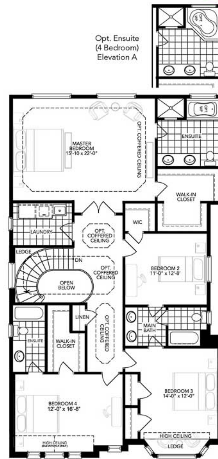
Opt. Second Floor (4 Bedroom) Elevation A
