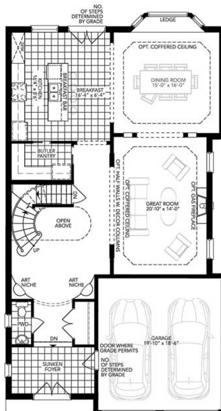
Opt. First Floor Elevation A
