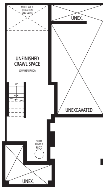
CRAWL SPACE
