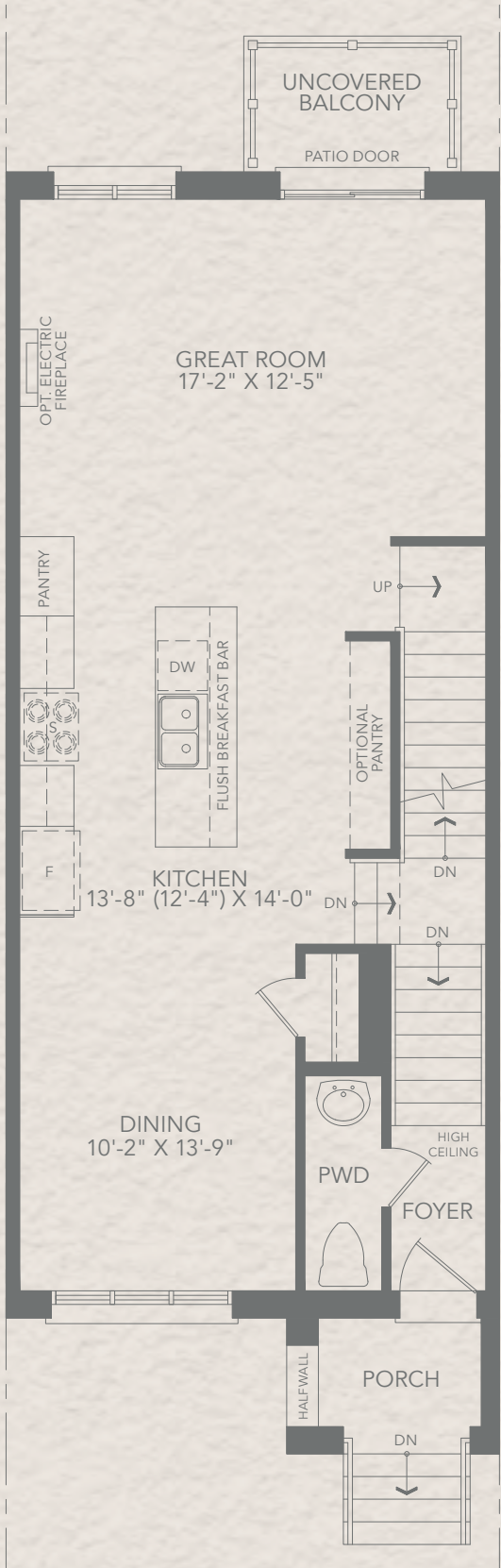
MAIN FLOOR PLAN EL. A2
