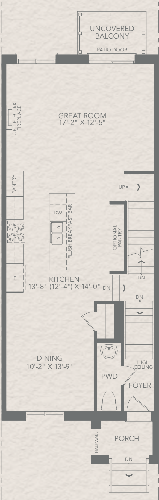
MAIN FLOOR PLAN EL. A3
