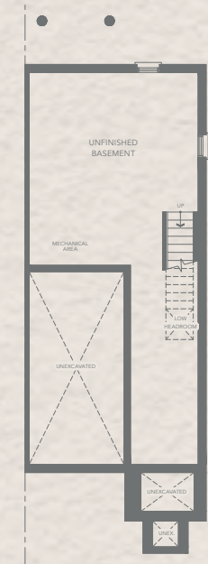
BASEMENT PLAN EL. A2 MOD
