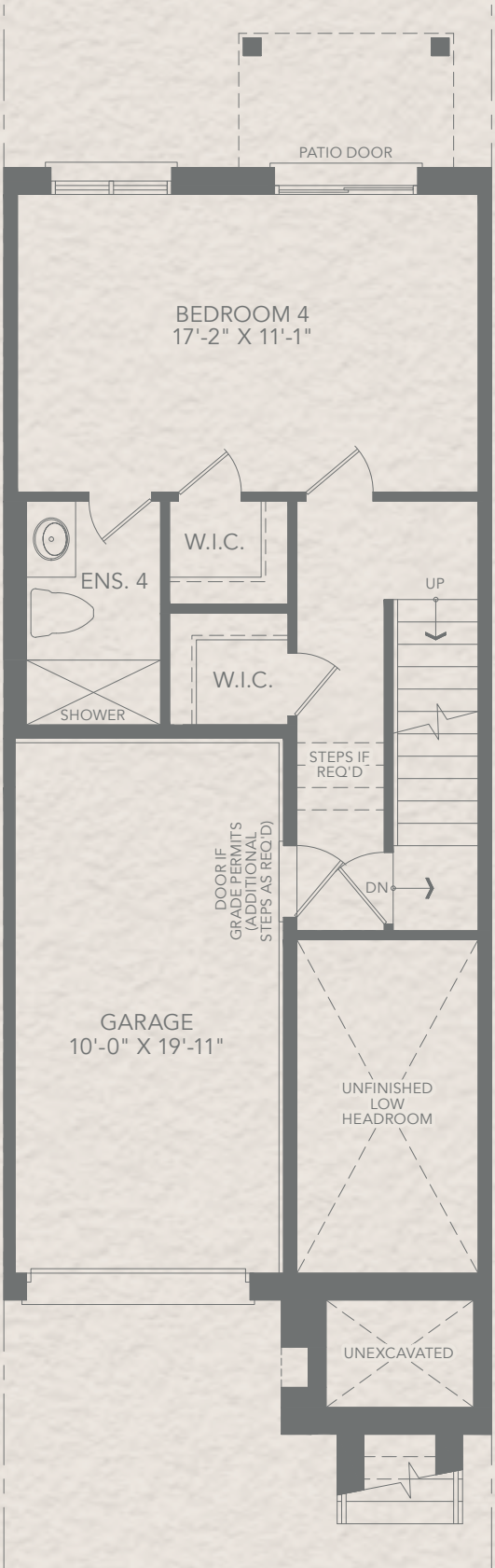
OPT. GROUND FLOOR PLAN EL. A1
