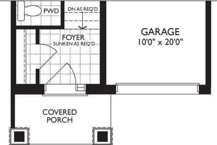
PART. MAIN LEVEL - ELEV. B
