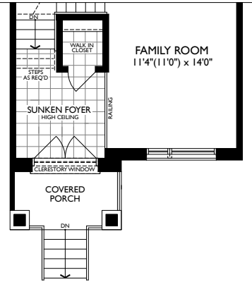
PART. OPT. MAIN LEVEL - ELEV. B
