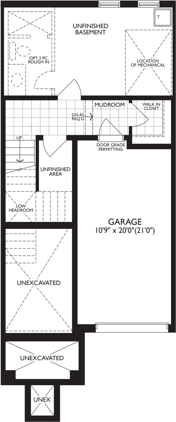
GROUND LEVEL - ELEV. A & B
