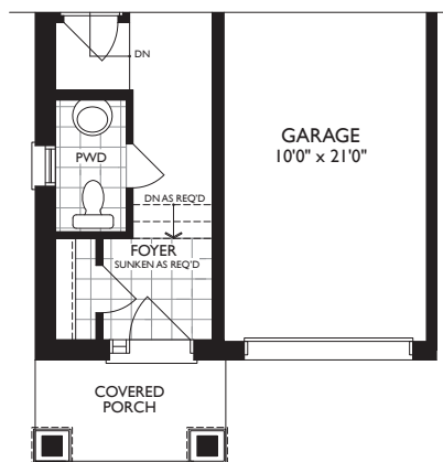
PART. MAIN LEVEL - ELEV. B
