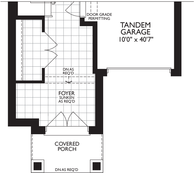
PART. OPT. GROUND LEVEL W/TANDEM GARAGE - ELEV. C
