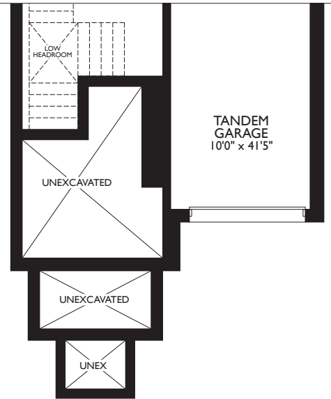
PART. OPT. GROUND LEVEL W/TANDEM GARAGE - ELEV. C
