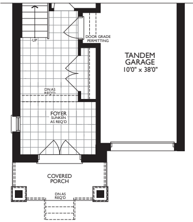
PART. OPT. GROUND LEVEL W/TANDEM GARAGE - ELEV. B
