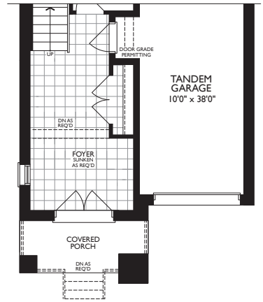
PART. OPT. GROUND LEVEL W/TANDEM GARAGE - ELEV. C
