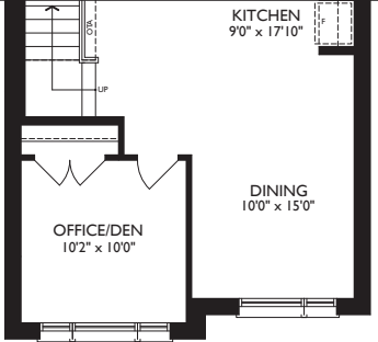
PART. MAIN LEVEL - ELEV. B
