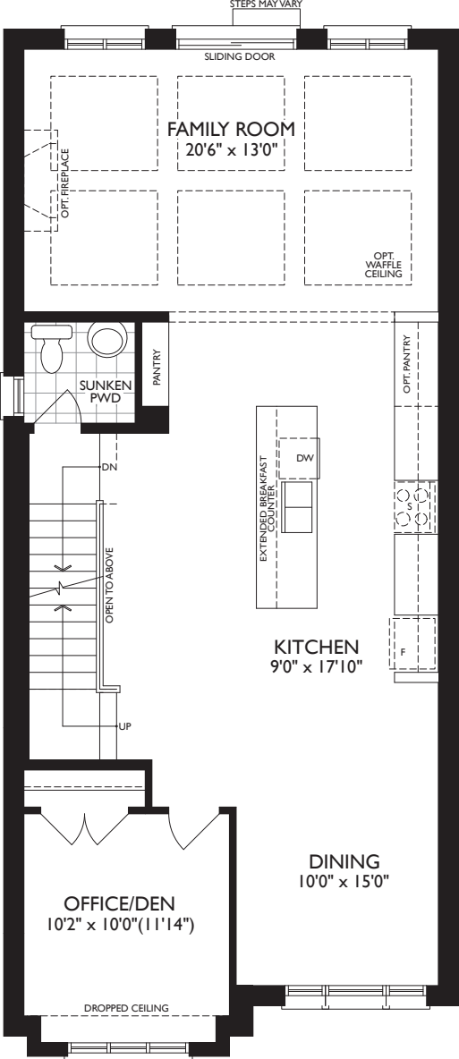
MAIN LEVEL - ELEV. A
