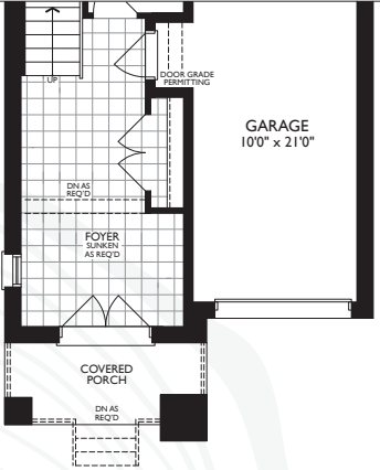
PART. GROUND LEVEL - ELEV. C
