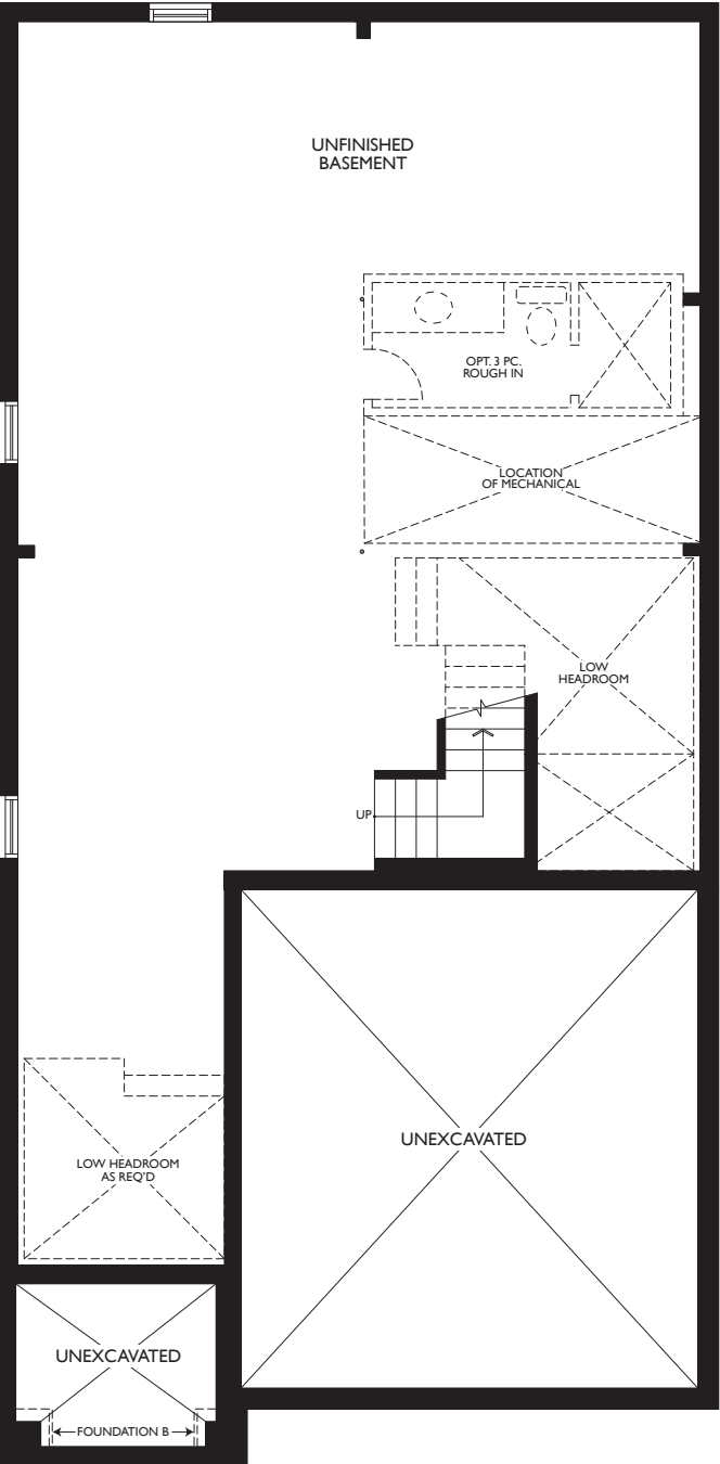
LOWER LEVEL - ELEV. A, B & C
