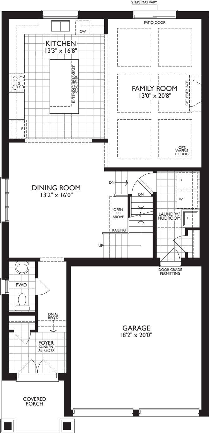
MAIN LEVEL - ELEV. A
