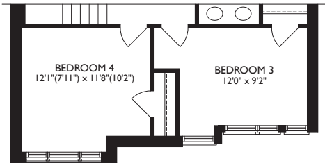
PART. UPPER LEVEL - ELEV. C SIMILAR TO ELEV. B
