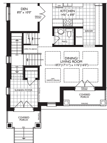
PART. MAIN LEVEL - ELEV. C
