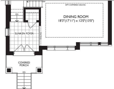
PART. MAIN LEVEL - ELEV. C
