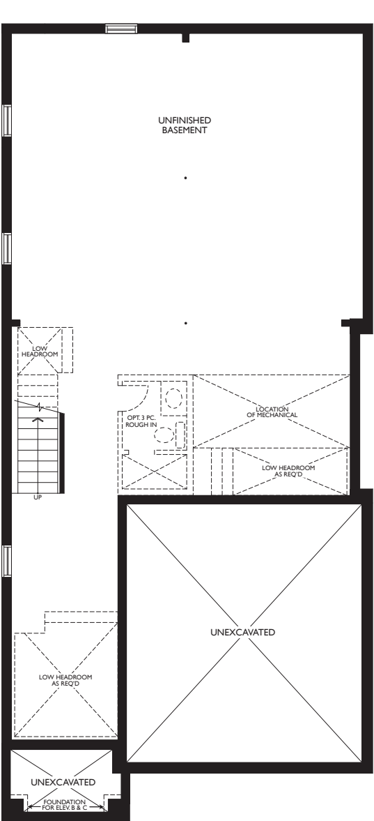
LOWER LEVEL - ELEV. A, B & C
