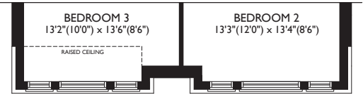
PART. UPPER LEVEL - ELEV. C
